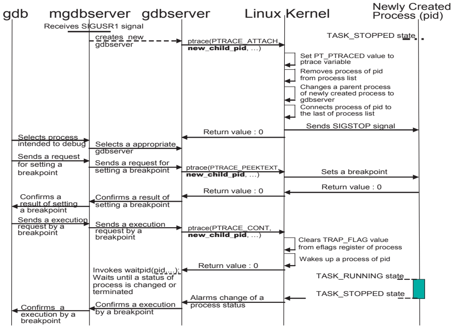
Fig. 2. Flow of debugging newly created process after mgdbserver receives signal
