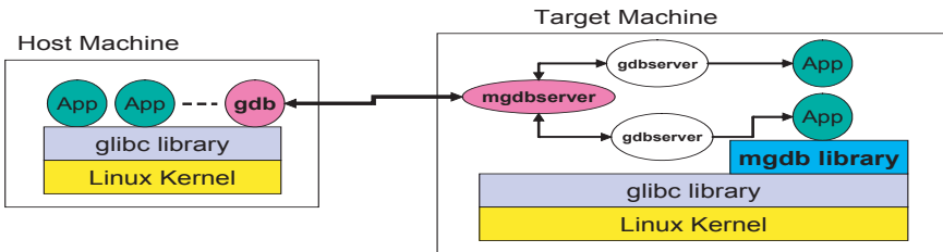
Fig. 1. Overview of our concurrent and remote debugging mechanism
