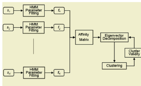
Fig. 1. Flow diagram of clustering sequences.
