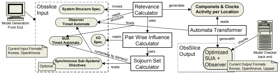
Fig. 1. OBSLICE architecture
