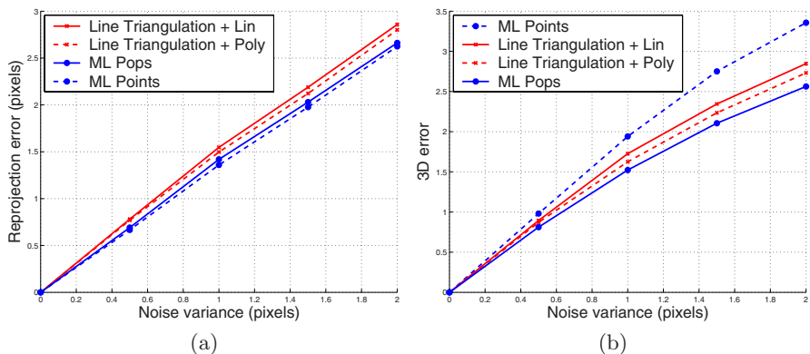
Fig. 3. Reprojection and 3D error when varying the added image noise variance to compare structure and motion recovery methods.
