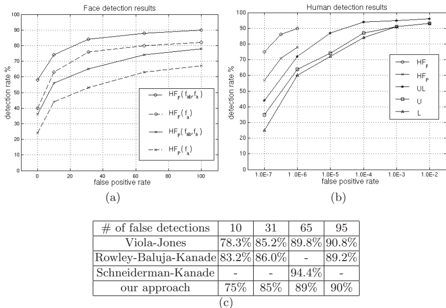
Fig. 5. (a) ROC curves for face detectors. HF_F(f_a) are the results for combined frontal head H and face F detector using single features f_a . HF_F(f_{ab}, f_a) are the results for the detector using both single features and feature pairs. Similarly for the profile detector HF_P . (b) ROC curves for head/face, upper body and legs detectors. The results for head/face are converted from HF(f_{ab}, f_a) displayed in figure (a). U are the results for individual upper body detector and L for the individual legs detector. U|L are the results for upper body detector combined with legs detector. (c) Face detection results compared to state of the art approaches.
