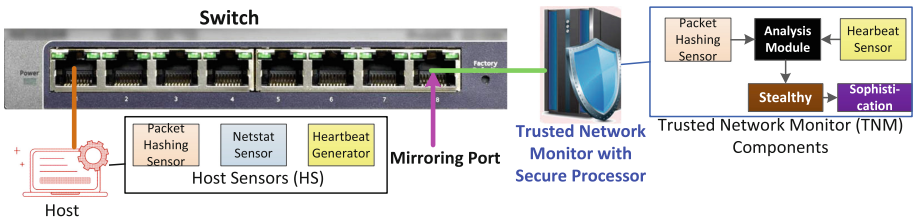
Fig. 1. Multi-level monitoring method: Uses host sensors (HS) and the Trusted Network Monitor (TNM)
