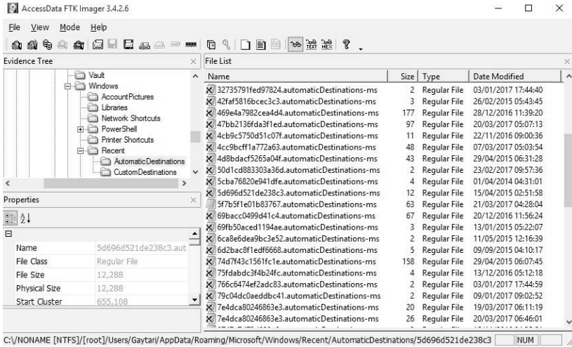
Figure 4. Deleted jump lists shown in FTK Imager.
