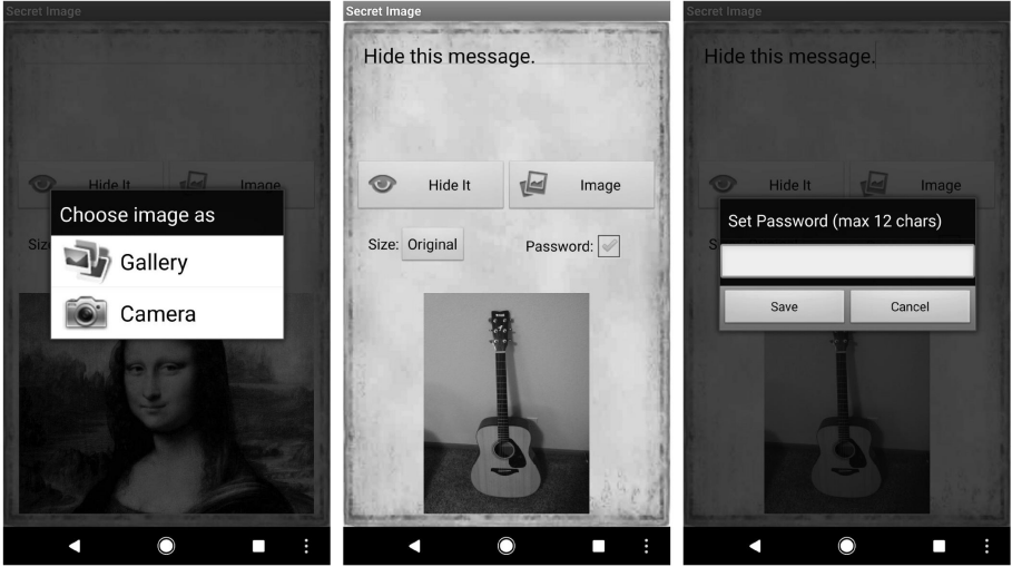
Figure 2. User input sequence for the Da Vinci app.
