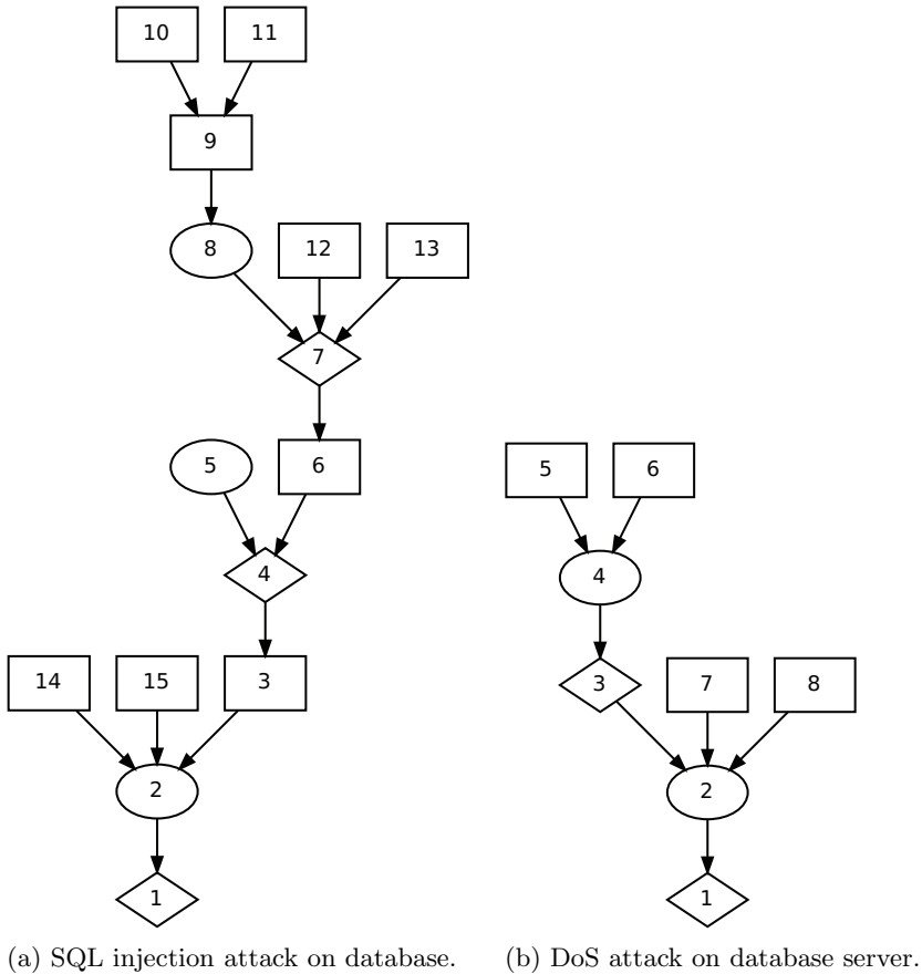
Figure 8. SQL injection attack and DoS database attack LEGs.
