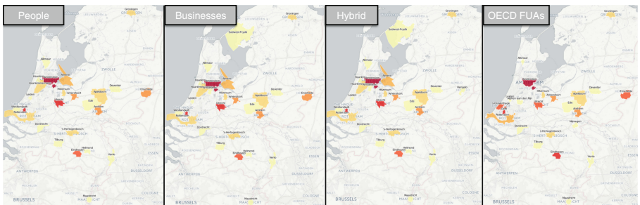
Fig. 8. Amount of RVO project subsidies mapped to the dynamically delineated FUAs defined based on the CBS open statistical data and OpenStreetMap boundaries.
