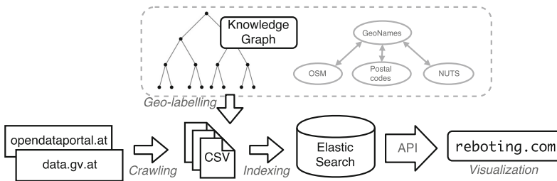
Fig. 1. Process of crawling, labelling, indexing and visualizing datasets from the Austrian Open Data portals.
