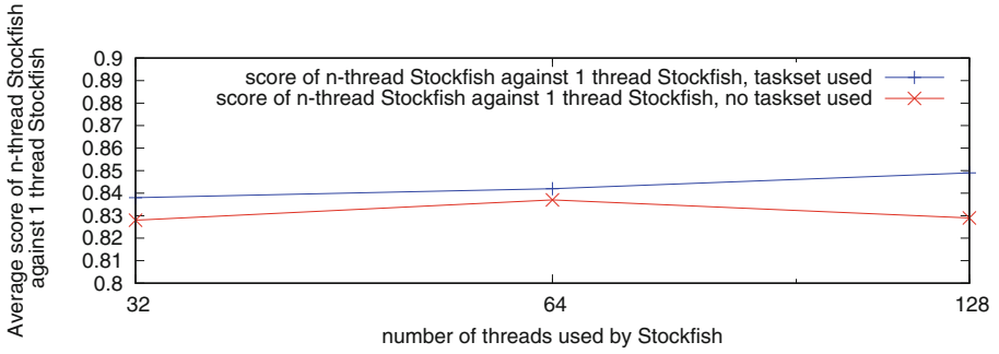
Fig. 2. How using taskset affects performance on Intel Xeon Phi x200
