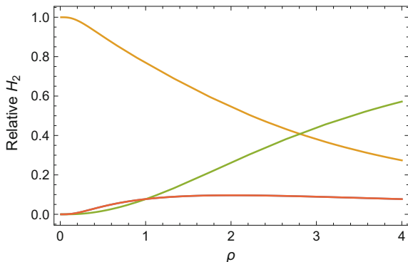
Fig. 6.2 Relative \mathcal{H}_2 values for the transfer functions in Eq. 6.1, with G_{ud} = G_{\eta n} in red, G_{nd} in gold, and G_{un} in green. The \mathcal{H}_2 value for each transfer function is divided by the total \mathcal{H}_2 values over all four functions. The transfer functions were derived from the process in Eq. 6.8 and the associated optimal controller. The weighting parameters in the cost function of Eq. 6.4 are \mu = 1 and \rho varying along the x -axis of the plot. Swapping values of \mu and \rho gives identical results, because of the symmetries in Eqs. 6.1 and 6.4
