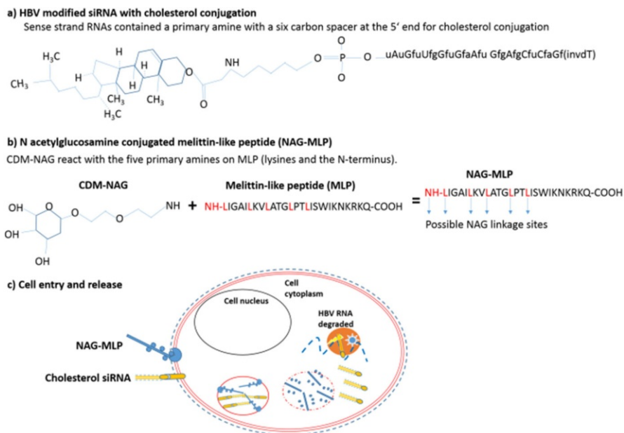
Fig. 14 ARC520. a A co-administered modified cholesterol-conjugated siRNA and b NAG-MLP polymer. c Both components are endocytosed by the respective receptors. In the acidic endosome, NAG is released and MLP is able to associate and disrupt the endosome membrane. This allows siRNA to be released into the cytoplasm, where it can associate with RISC, leading to HBV RNA degradation
