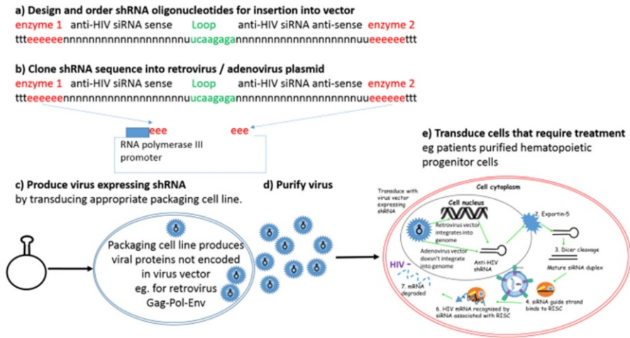
Fig. 12 Development of viral vectors. a Design the shRNA sequences required using online algorithms and oligonucleotide companies; b clone shRNA oligonucleotides into the commercially available viral vector plasmid that suits the expression profile required; c transfect plasmids into specialised commercially available packaging cell lines that produce the replication factors required for the specific virus vector; d purify the virus that is produced, and e transduce the cells that require treatment
