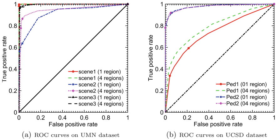
Fig. 3. The ROC curves for the detection of GAE on the UMN dataset.
