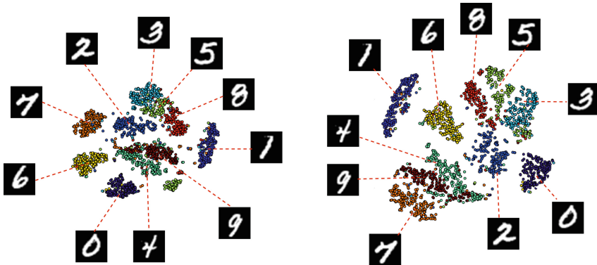
Fig. 4. Backprop ( Left ) and crossprop ( Right ) seem to learn similar feature representations, by clustering together similar examples. The plot shows the visualizations of the features (i.e. activations of the hidden units) learned by backprop and crossprop on the standard MNIST task. Both the learning algorithms were trained online on the MNIST dataset and the parameters learned by these algorithms were used for generating these visualizations. The \eta was set to 0 for crossprop in order to draw out differences between the conventional and the meta-gradient descent approach for learning the features. The plot was generated by using 2500 training examples, uniformly sampled from the MNIST dataset.
