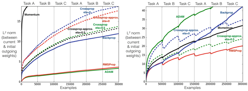
Fig. 3. Left: generated from GEOFF tasks. Right: generated from MNIST tasks. The plots show the change in the outgoing weights W after processing each example. It shows the l^2 norm between the outgoing weights W after processing the n^{\text{th}} example and its initialized value for different learning algorithms. From the plots, it can be observed that crossprop tends to change the outgoing weights the most as it is needed to map the feature representation to an estimate y_t . In backprop, each parameter independently minimizes the error and because of this, each parameter race with each other in reducing the error without coordinating their efforts. So, it tends to change its feature representation for accommodating a new example.
