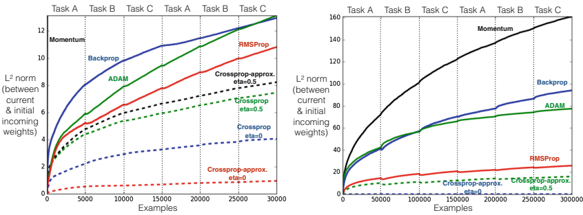
Fig. 2. Left: generated from GEOFF tasks. Right: generated from MNIST tasks. The plots shows the change in the incoming weights U after processing each example. Specifically, the plots shows l^2 norm between the incoming weights U after processing the n^{\text{th}} example and its initialized value for different learning algorithms. From the plots, it can be observed that crossprop tends to change the incoming weights the least even when the task is significantly changed, implying that crossprop tends to find a reusable feature representation that can sufficiently solve the sequence of tasks that it experiences. On the other hand, backprop tends to significantly relearn the feature representation throughout the experiment even when the task can be solved by leveraging from previous learning experiences.
