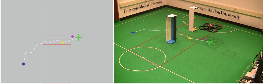
Fig. 3. Left: A 2-D visualization generated from the interesting events of one run of the RRT, using a domain based on physical obstacles. Right: The result of drawing that visualization onto the corresponding frame from the video of the real robot.
