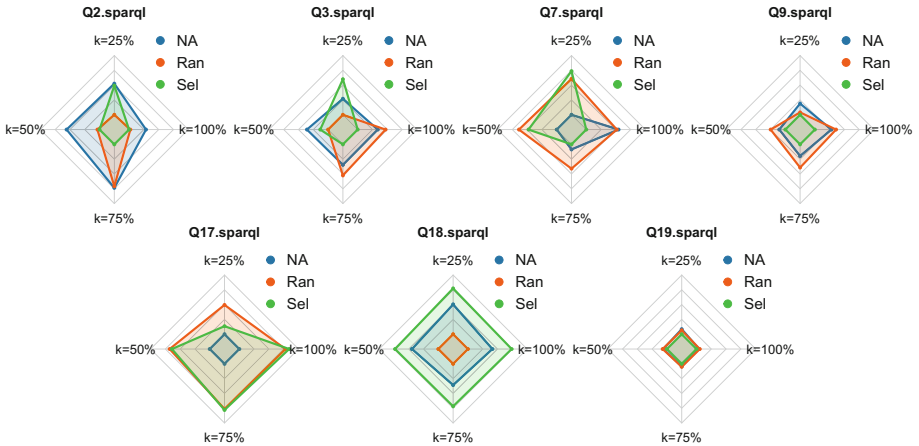
Fig. 6. Diefficiency while producing a portion k of the answers, per benchmark query and SPARQL query processing approaches: nLDE Not Adaptive (NA), nLDE Random (Ran), nLDE Selective (Sel). Performance is measured with dief@k , with k = 25\% , k = 50\% , k = 75\% , k = 100\% . Interpretation of the axes: lower is better.
