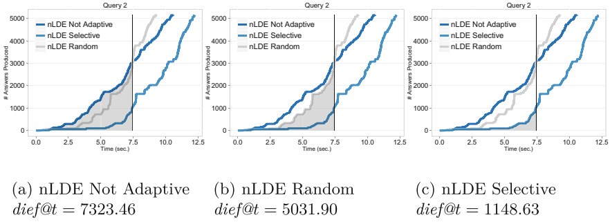
Fig. 3. dief@t of the nLDE engine for Query 2 at t = 7.45 . (a), (b), and (c) highlight the area under the curve of the answer distribution function that is computed for measuring the diefficiency of the approaches at the given t . nLDE Not Adaptive exhibits the best performance for the given interval, followed by nLDE Random and lastly nLDE Selective. The reported dief@t values are congruent with these observations.
