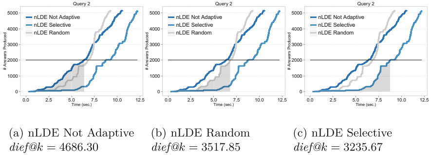
Fig. 4. dief@k of the nLDE engine for Query 2 at k = 2000 . (a), (b), and (c) highlight the area under the curve of the answer distribution function that is computed for measuring the diefficiency of the approaches while producing the first k answers. The slope of the answer distributions indicate that nLDE Selective produces the first 2000 answers at a higher rate, followed by nLDE Random and then by nLDE Not Adaptive. The reported dief@k values are congruent with these observations.
