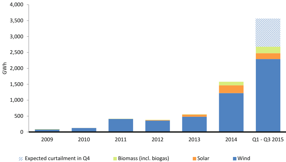
Fig. 1. Development of curtailed energy between 2009 and 2015 in Germany [GWh] [8–10] (At the time of writing the curtailment of quarters one through three of 2015 were published. The dashed form approximates our expected curtailment in quarter four (Q4) of 2015.)
