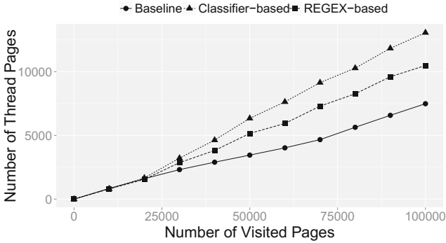
Fig. 7. Performance of the 3 strategies of intra-site crawling.
