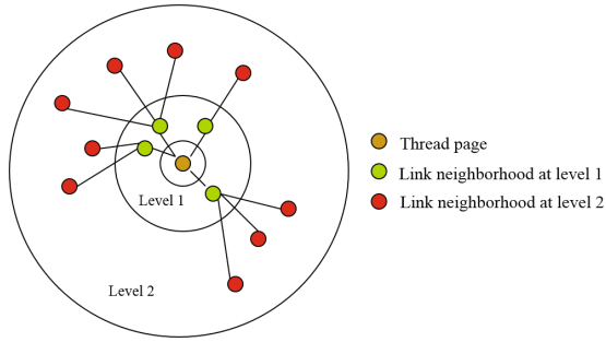
Fig. 5. Example of context graph for thread pages (adapted from [6]).
