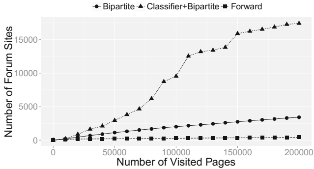
Fig. 4. Performance of the 3 strategies of inter-site crawling.
