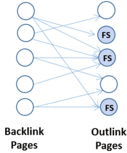
Fig. 3. Example of bipartite graph used by the Inter-Site crawler to locate forum sites (FS stands for forum sites).
