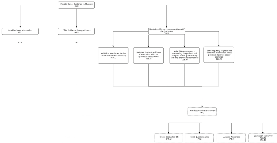
Fig. 3. Goal model
