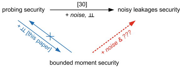
Fig. 7. Reductions between leakage security models.
