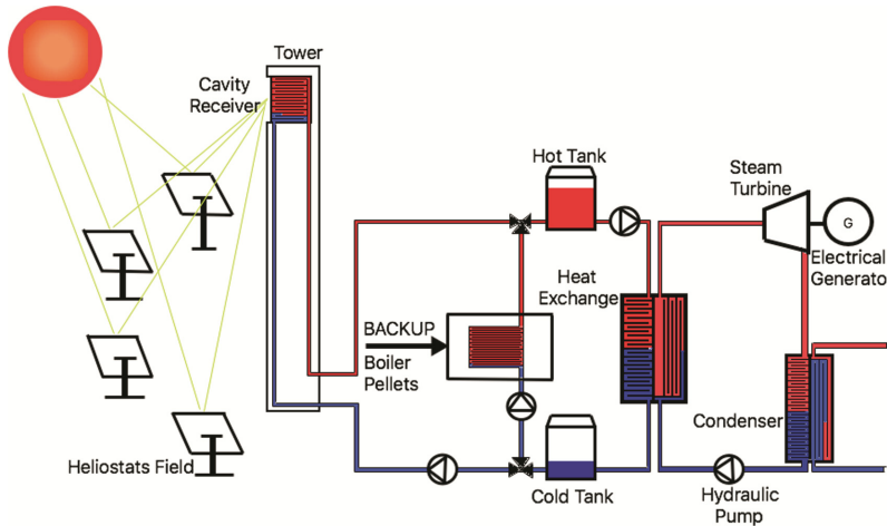
Fig. 3. Operating principle of the solar thermoelectric tower with back-up with biomass.
