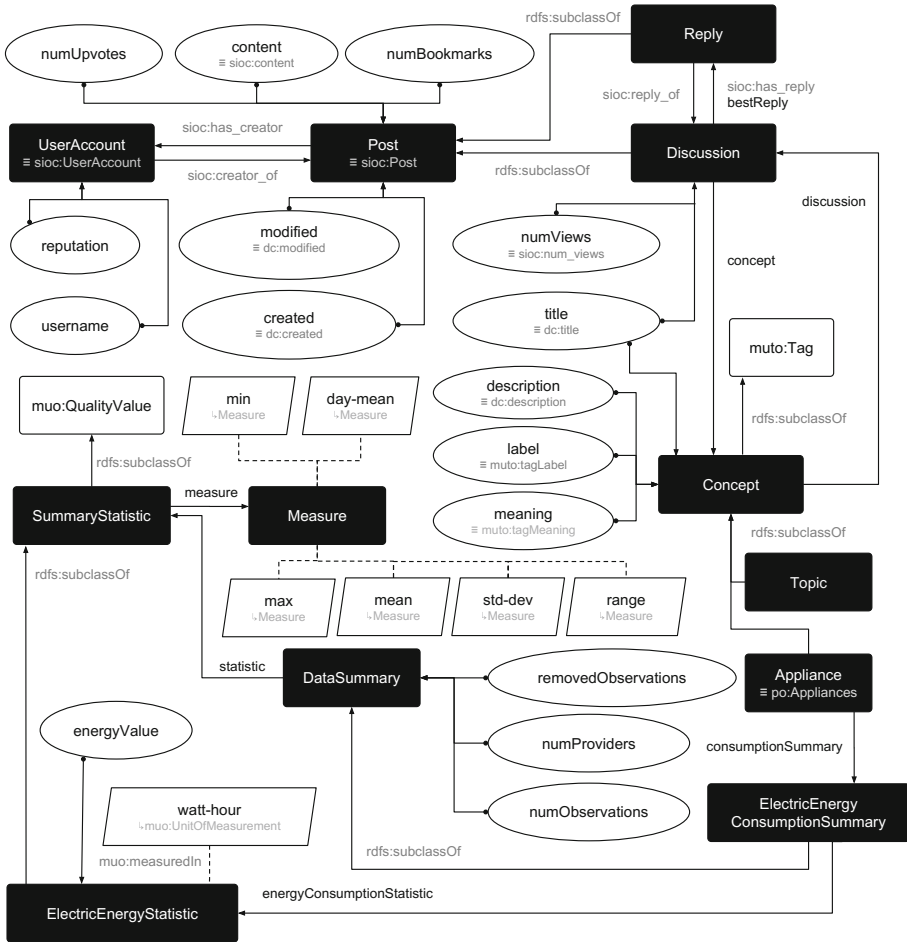
Fig. 4. EnergyUse ontology, which imports properties and classes from 6 ontologies: SIOC [4] (sIOC), PowerOnt (po), MUTO (muto), DC Terms (dc), FOAF (foaf) and MUO (muo). Rectangles denote classes, ellipses properties, and parallelograms class instances.
