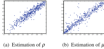
Fig. 4. Visualization of synthetic data experiment on inference of partition parameters \rho and \mu . The x-axis is the ground truth and the y-axis is the estimation. Each dot in the plot presents the \rho and \mu for a document (a) Estimation of \rho (b) Estimation of \mu
