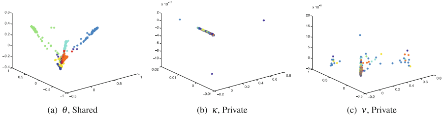
Fig. 5. Visualization of the shared topic representation ( \theta ) and private topic representations ( \kappa and \nu ) for LabelMe experiments using randomly paired images from the same class. The documents of different classes are colored differently and the plots show the first three principal components after applying PCA on the per document topic distributions for all the training data. (Color figure online)
