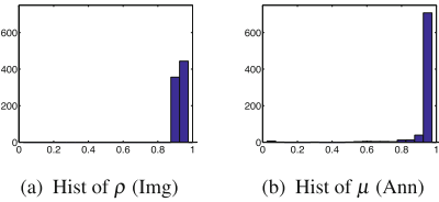
Fig. 7. The histogram over partition parameters of the LabelMe image-annotation experiment. Img indicates that this modality uses natural images. Ann indicates that this modality uses image annotations (a) Hist of \rho (Img) (b) Hist of \mu (Ann)
