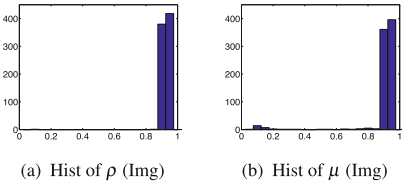
Fig. 6. The histogram over partition parameters of the LabelMe image-image experiment. Img indicates that this modality uses natural images (a) Hist of \rho (Img) (b) Hist of \mu (Img)
