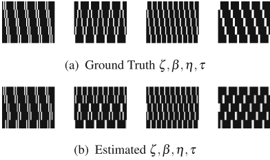
Fig. 3. (a) shows the ground truth of the four per topic word distributions in the two-view IBTM model; (b) shows the inferred distributions. Each row in the distributions represents a topic and each column presents a word. There are 5 topics in each distribution ( K = T = S = 5 ), and the vocabulary size is 50 for both views ( V = W = 50 ) (a) Ground Truth \zeta, \beta, \eta, \tau (b) Estimated \zeta, \beta, \eta, \tau
