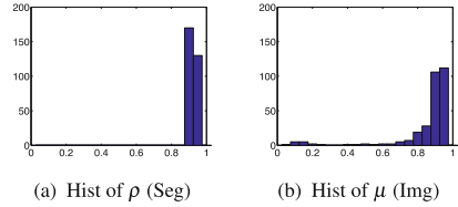
Fig. 11. The histogram over partition parameters of the Leeds Butterfly image-segmentation experiment. Img indicates that this modality uses natural images. Seg indicates that this modality uses segmented images (a) Hist of \rho (Seg) (b) Hist of \mu (Img)
