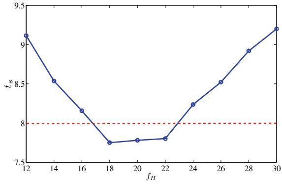
Fig. 5.16 Effect of packet collision phenomena on the algorithm performance: algorithm settling time t_s versus f_H
