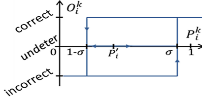
Fig. 1. The update rule of the opinion
