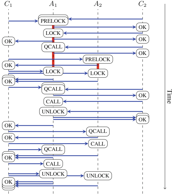
Fig. 3. All three phases: a process on C_1 calls transfer on A_1 and A_2 ; a process on C_2 concurrently calls withdraw on A_1
