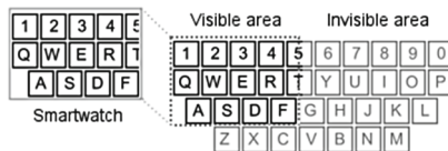
Fig. 1. The Virtual Sliding QWERTY (VSQ). To enter a character with this technique, the user drags the keyboard to a particular region and then taps on the intended key.
