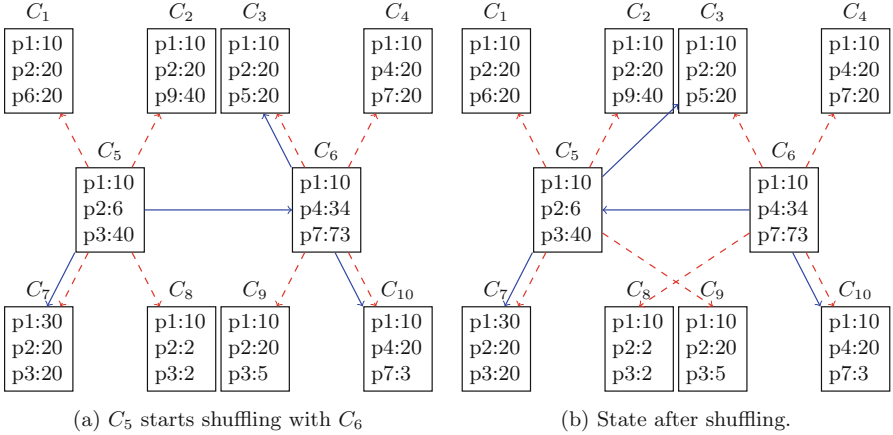
Fig. 2. Partial CyCLaDEs network centered on $C_5, C_6$. Solid lines represent clients in RPS view (2). Dashed lines represent clients in CON view (4). Each client has a profile size of 3 defined as predicate : frequency .
