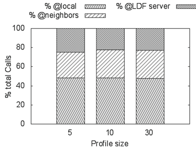
Fig. 5. Impacts of profile size on hit-rate for two datasets with 50 clients per dataset. RPS_{view} = 6 and CON_{view} = 15 . Profile_{size} = 5, 10 and 30
