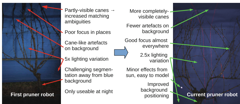
Fig. 7. Hardware changes have improved several different aspects of the vine images from the first pruner robot to the current system.
