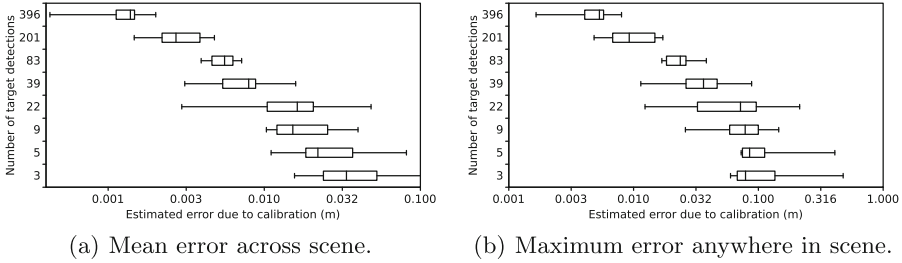
Fig. 5. Effect of the number of targets detected in both images of a stereo pair on the accuracy of reconstructed 3D points. Box plots show the range, quartiles, and median errors, from 15 calibrations for each number of targets. The scene is 2 m wide, with a depth of field of 0.5 m to 1.75 m.
