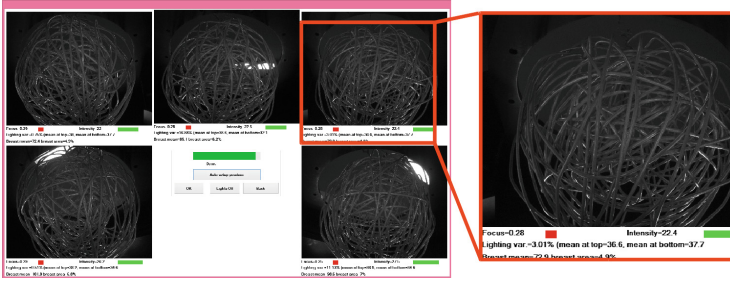
Fig. 4. The DIET machine’s GUI for setting camera focus. The wire ball has sharp edges at a range of depths. The focus and aperture are set to maximise the sum of squared differences between neighbouring pixels.
