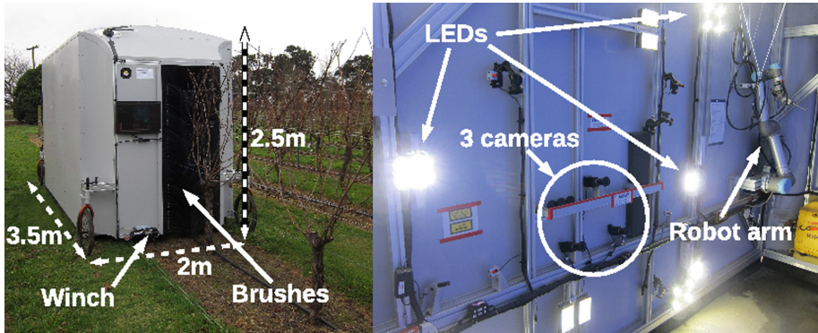
Fig. 1. The pruner robot's mobile platform completely covers the vines, blocking out sunlight (left). Inside are high-powered LEDs, three cameras, a robot arm, a generator and the desktop PC that runs all of the software (right).
