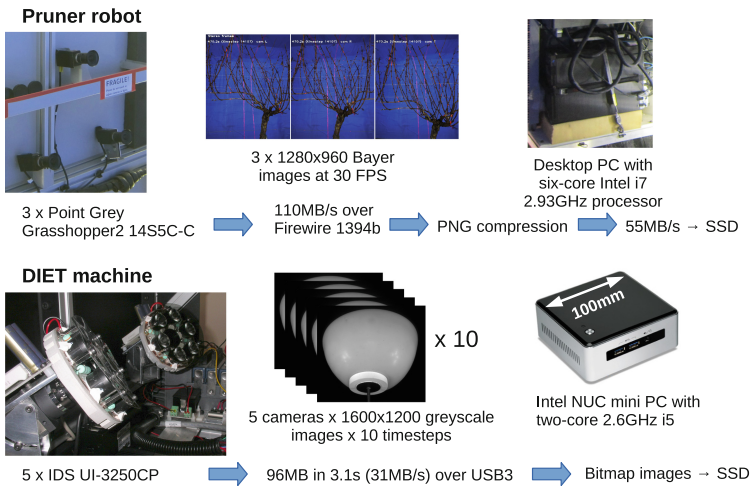
Fig. 3. Examples of image acquisition hardware setups. Modern USB3 and 1394b cameras allow high data-rate uncompressed imaging without specialised hardware (i.e. capture cards).
