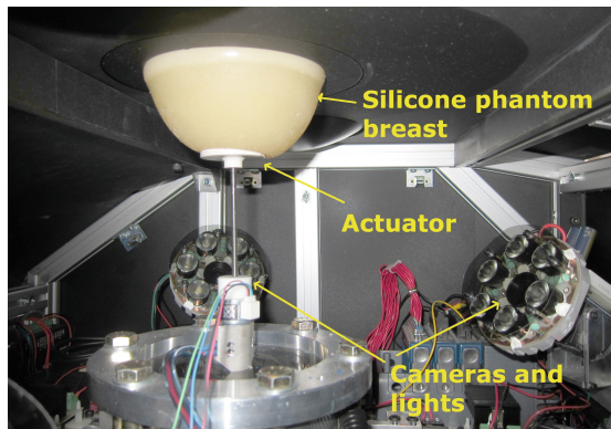
Fig. 2. The DIET machine, showing two of the five cameras, the actuator, and a silicone phantom breast. The machine measures 80 cm by 71cm by 38cm.
