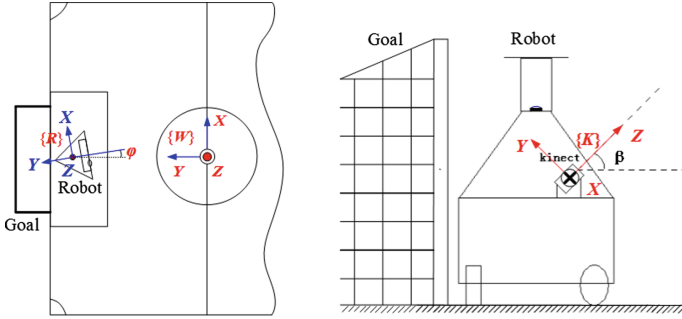
Fig. 3. The world coordinate system \{W\} , robot coordinate system \{R\} and the Kinect coordinate systems \{K\} .
