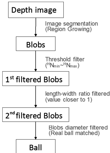
Fig. 5. The ball detection process with depth information.
