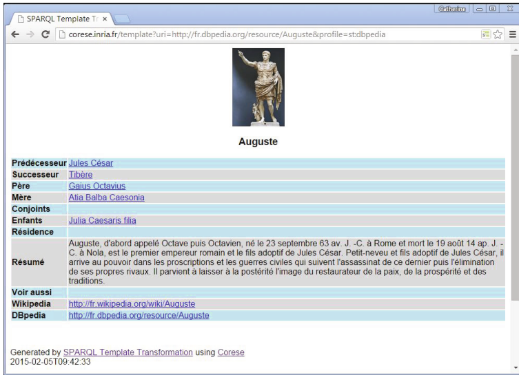
Fig. 2. DBpedia Navigator
