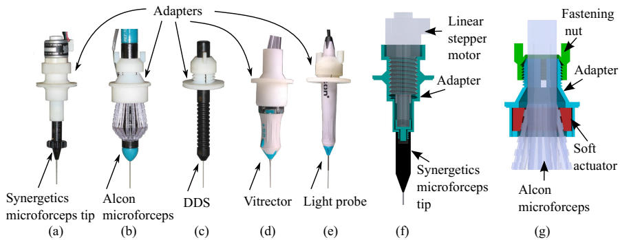
Fig. 2. (a)–(e) Disposable retinal-surgery instruments with adapters than enable quick-change mounting to the 6-DOF manipulator. (f) Section view of the Synergetics microforceps in (a) actuated by a linear stepper motor. (g) Section view of the Alcon microforceps in (b) actuated by a soft actuator.
