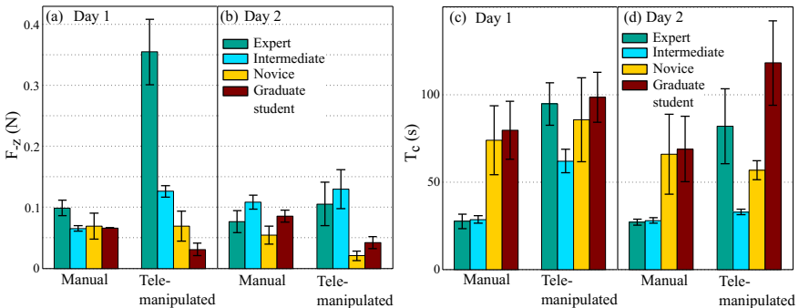
Fig. 3. Experimental results comparing manual and telesystem membrane peeling with a microforceps. (a)–(b) shows maximum downward force ( F_z ), and (c)–(d) shows completion time ( T_c ). Data is divided according to subject, day, and mode of experiment. Error bars indicate standard deviation.
