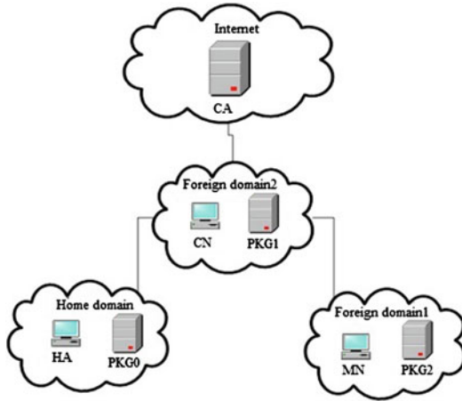
Fig. 2. Network Architecture
