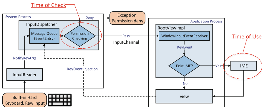
Fig. 5. Android KeyEvent processing framework and CAKI vulnerability
