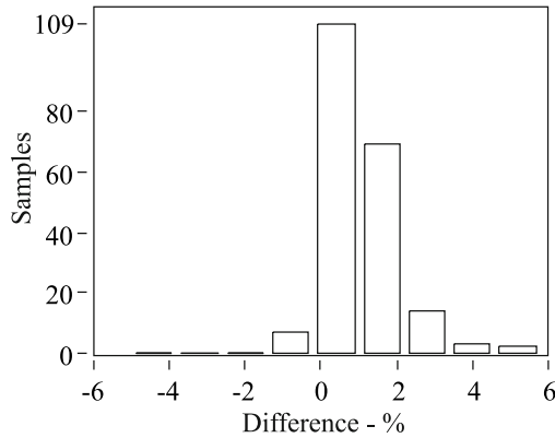
Fig. 13. ANN ensemble results
