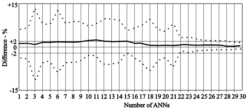
Fig. 10. Difference of refrigerating capacity versus number of ANNs
