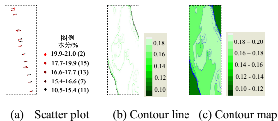
Fig. 7. Soil moisture distribution map
