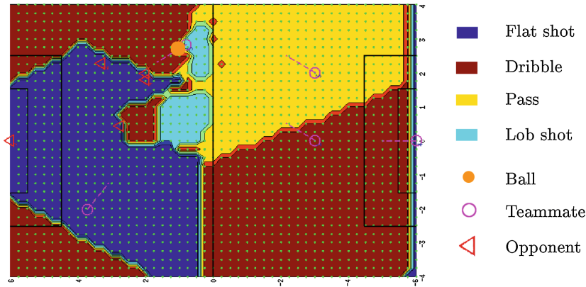
Fig. 5. Skill-selector visualization (Color figure online).
