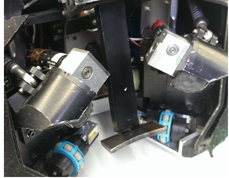
Fig. 4. Shooting lever end-effector for more accurate passing.
