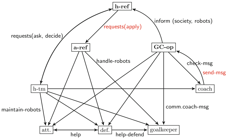
Fig. 1. Role dependency graph
