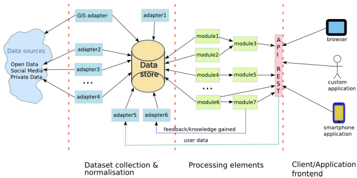
Fig. 1. Overall Design of KnowDS
