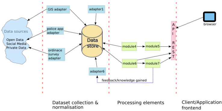
Fig. 3. UK Crime Application Design
