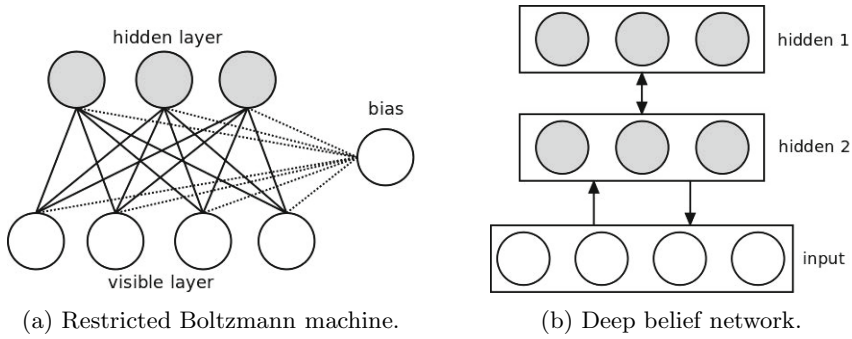
Fig. 1. Deep classifiers
