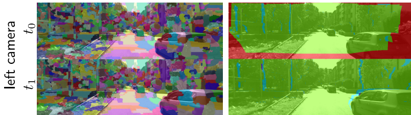
Fig. 4. Example from the KITTI training set (#191). (left) Consistent super-pixel segmentation (right) Active data term \varrho (Eq. 5). Colors denote normal photo-consistency (green), out of bounds (red), occluded (light blue), and implausible (dark blue).
