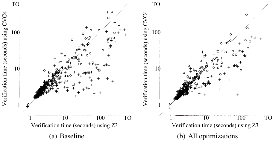
Fig. 3. Scatter plots comparing the performance of Z3 and CVC4 over the responsive benchmarks. A symbol +, respectively \circ , represents a kernel for which verification succeeds, respectively fails.
