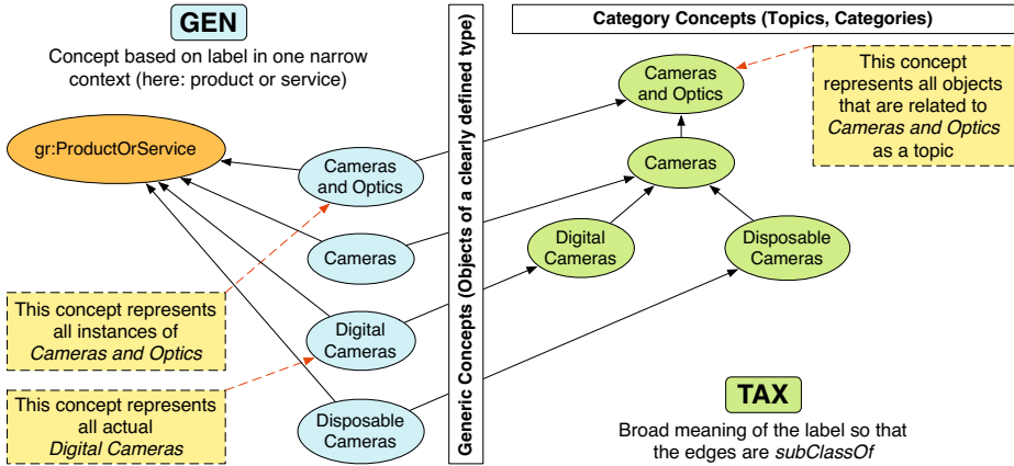
Fig. 2. GenTax applied on an extract of Google product taxonomy (cf. [20])
