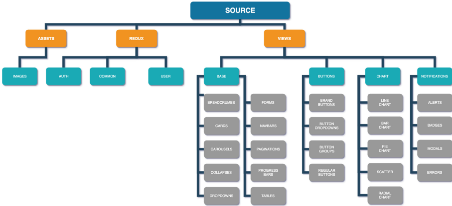
Fig. 3. File structure of the implementation
