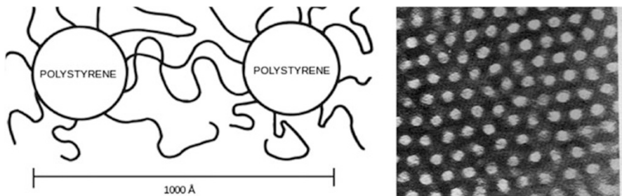
Fig. 3.5 Left: A scheme of separation of block copolymer units. Right: The resulting pattern
