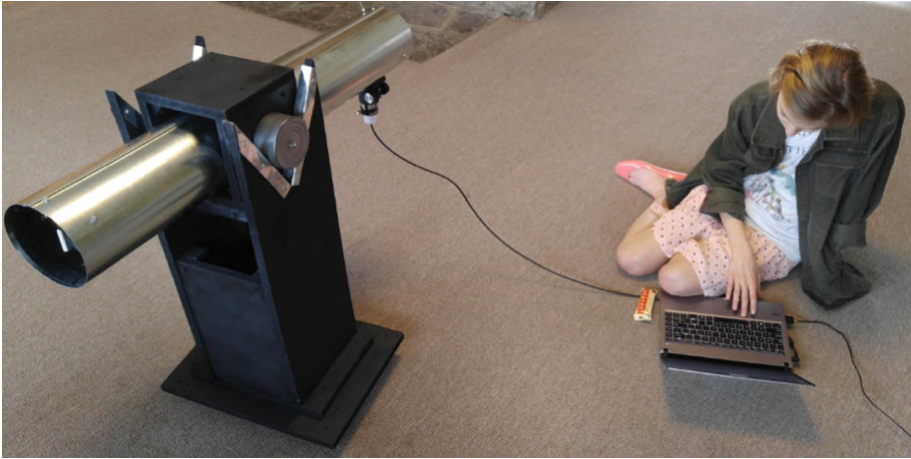
Fig. 2. This near-infrared telescope for SETI uses all gold first surface optics and a high speed InGaAs detector. An SDR connects the detector to the computer for data monitoring and collection.
