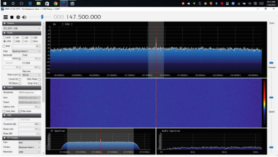
Fig. 5. A beacon-like signal with a more realistic intensity, but still lacking in Doppler shift (Color figure online)
