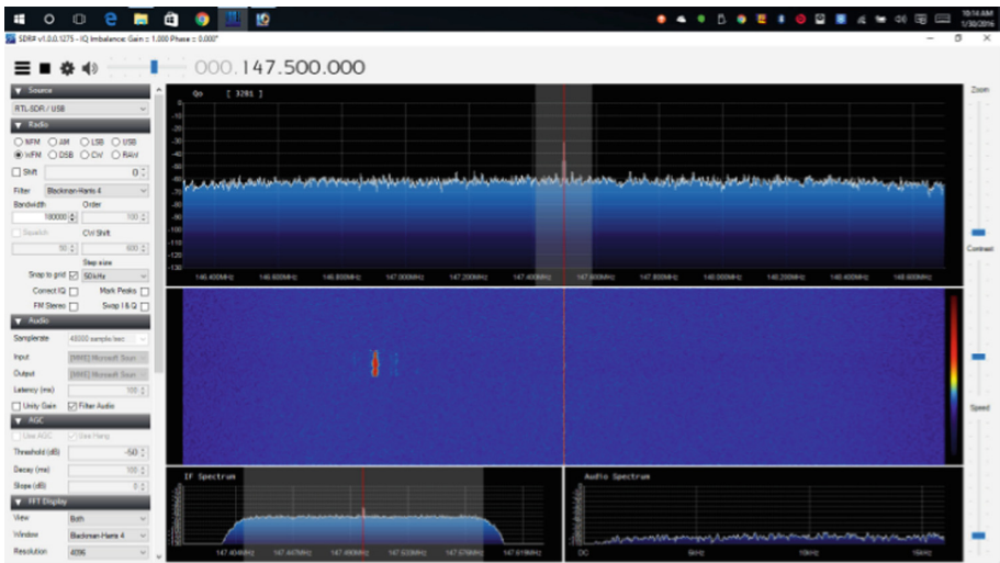
Fig. 4. A system test using frequency modulated light pulses. (Color figure online)
