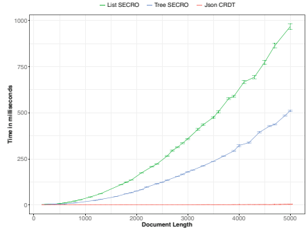
(b) Execution time of an operation that appends 100 characters to a document.
