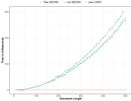
(a) Execution time of an operation that appends one character to a document.
