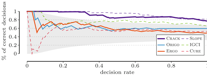
Fig. 3. [Higher is better] Decision rates of the multivariate methods \text{CRACK} , \text{ORIGO} and \text{ERGO} , and the univariate methods \text{IGCI} , \text{CURE} and \text{SLOPE} (dashed lines) on the univariate Tübingen causal benchmark pairs (100), weighted as defined.
